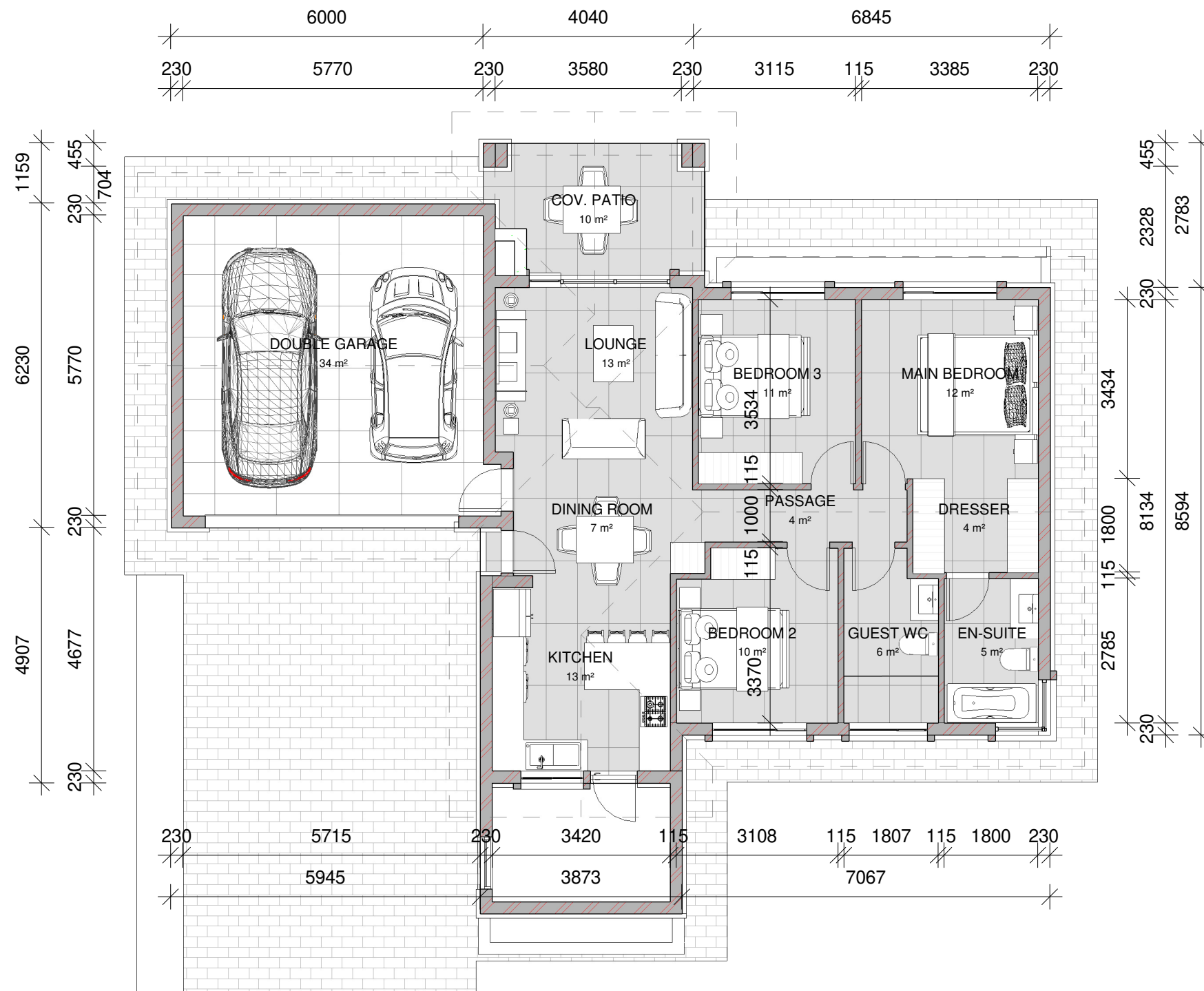
1 GROUND 1 : 100
